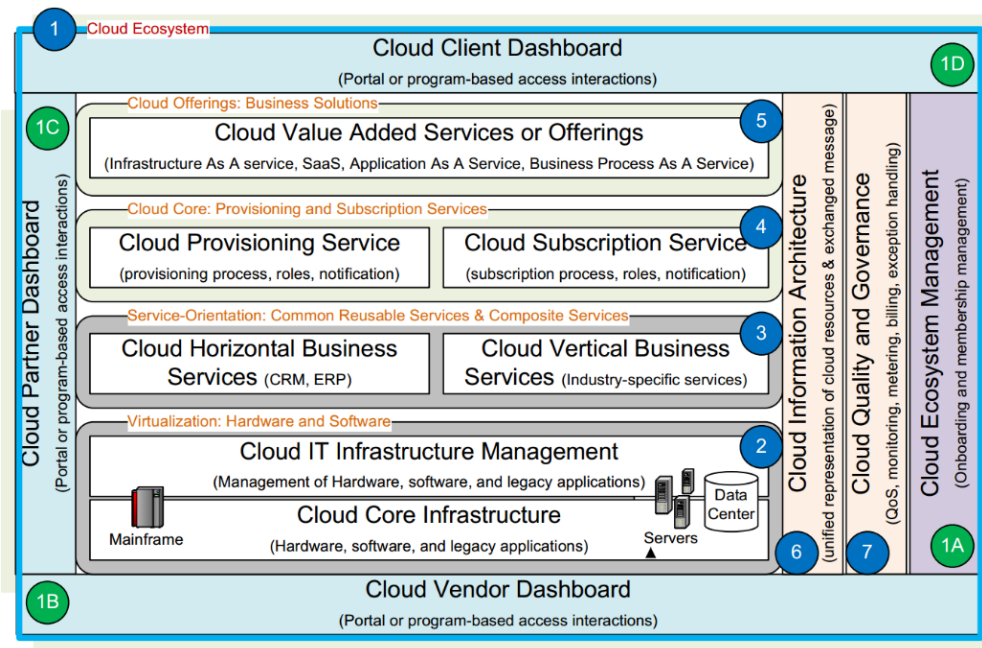
Figure 4. Open architecture of cloud computing [38]
