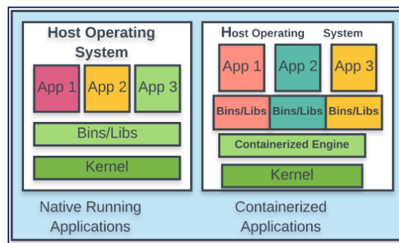
Figure 6. Native and containerized applications
