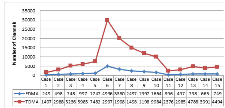
Figure 3. Number of Channels in TDMA & FDMA
