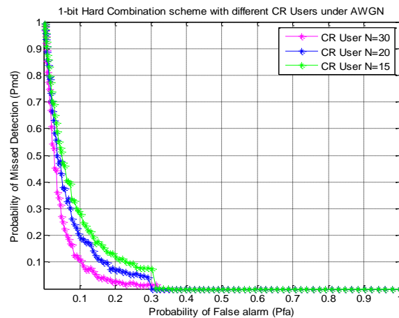
Figure 5. ROC of 1-bit OR rule with different CR users
