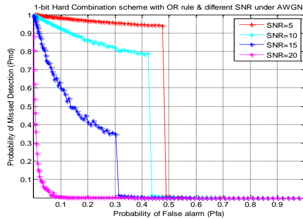
Figure 4 ROC of 1-bit OR rule with 10 CR users & different SNR
