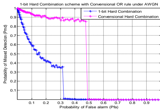
Figure 3. ROC of conventional and 1-bit OR rule with 10 CR users
