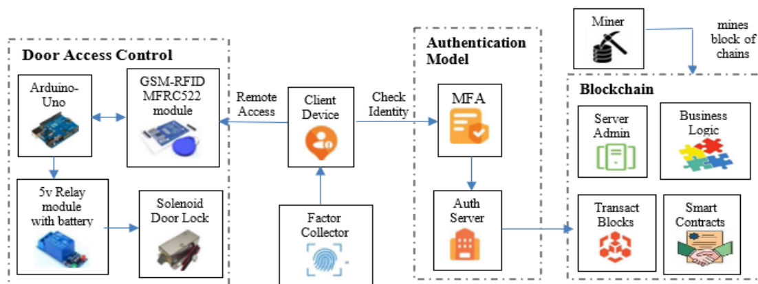
Figure 2. Schematic diagram of the proposed blockchain-MFA fused IoT solution
