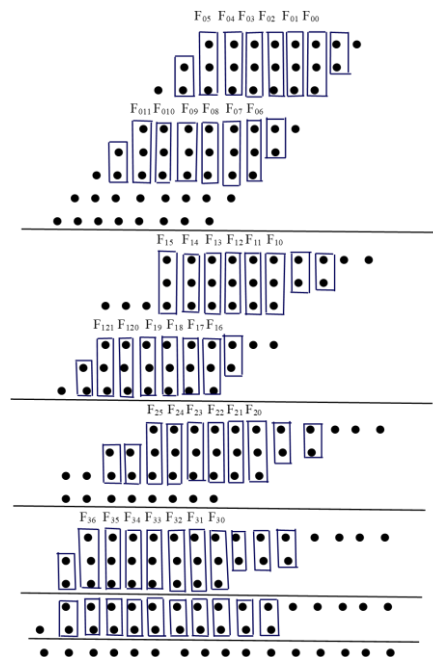
Figure 1. 8×8 Approximate wallace tree multiplier (AxWTM) using proposed AxAs
