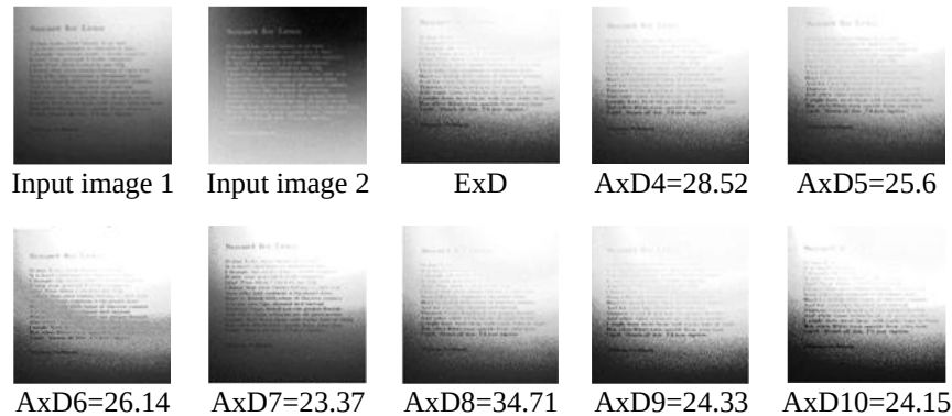
Figure 6. Image division
