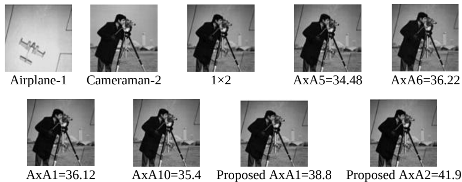
Figure 4. Image multiplication
