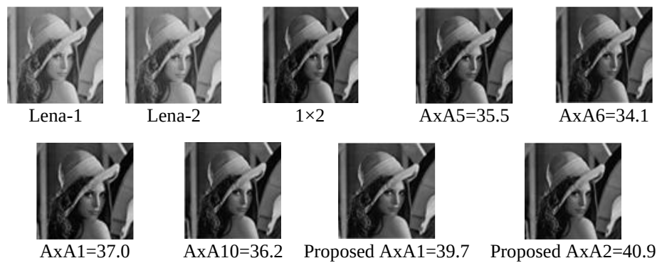
Figure 3. Image squaring
