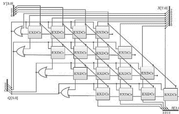
Figure 2. AxD using proposed AxSCs
