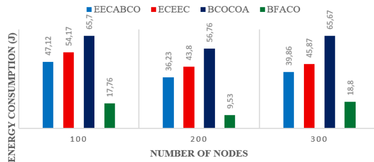
Figure 4. Comparative analysis of energy consumption nodes using BFACO with other research algorithms
