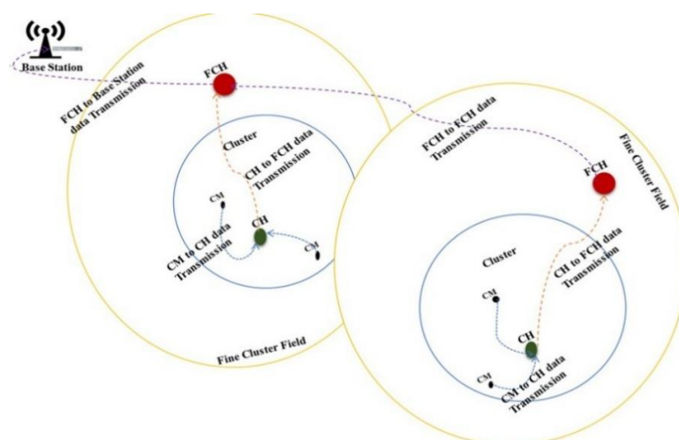
Figure 1. Organization of CMs, clusters with CHs, and fine clusters with FCHs in WSNs
