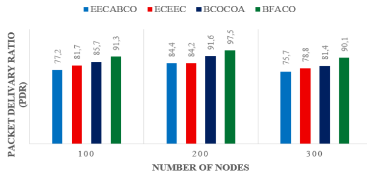
Figure 3. Comparison analysis of PDR using BFACO with other algorithms
