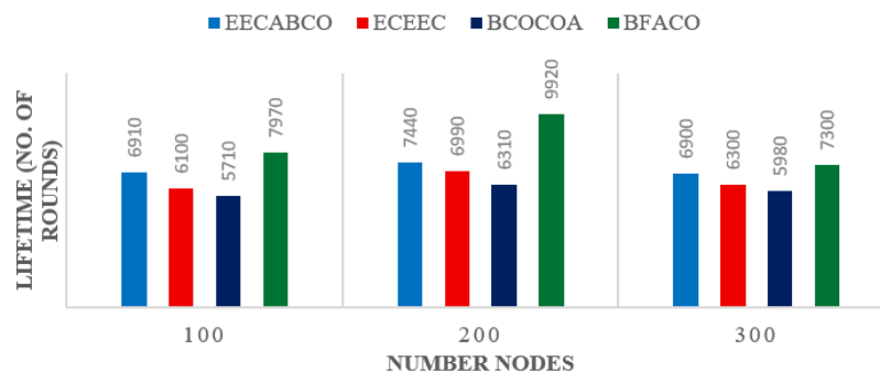
Figure 5. Comparative analysis of Lifetime of the network using BFACO with other research algorithms
