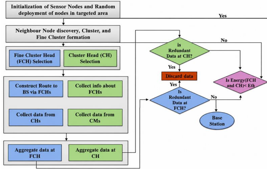
Figure 2. Process from initialization of nodes to sending data to Base Station (BS) using CHs, and FCHs
