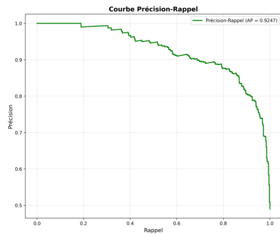
Figure 6. Accuracy-recall curve
