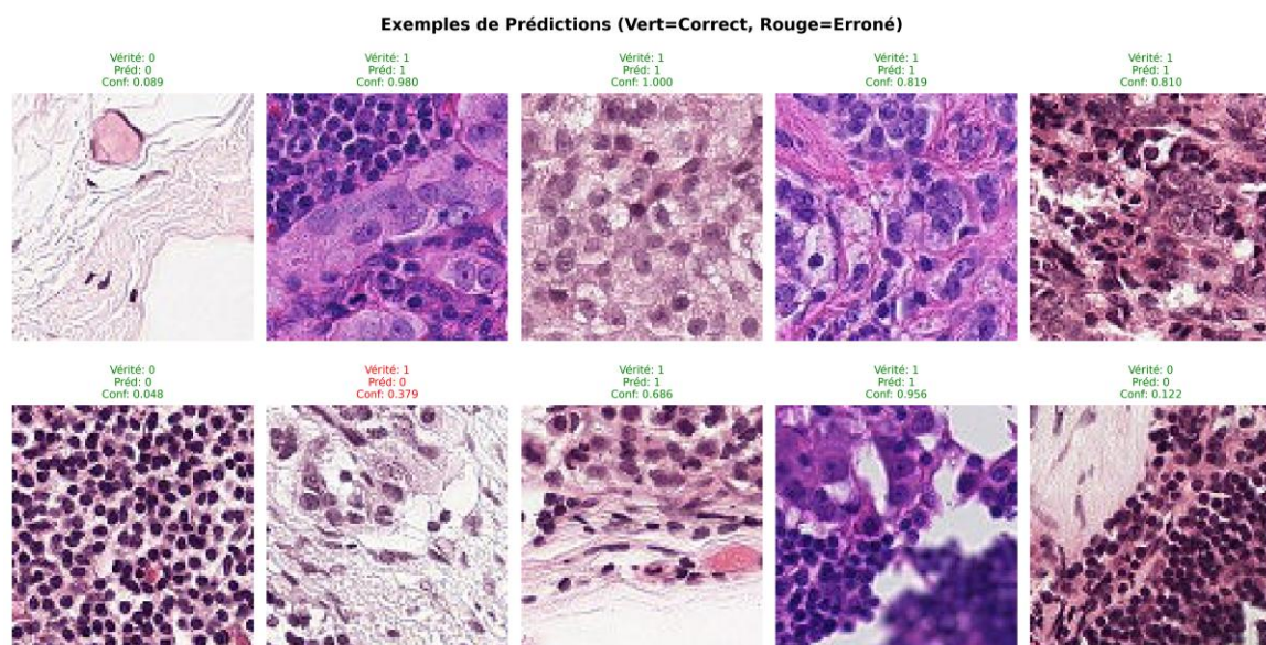
Figure 7. Sample predictions
