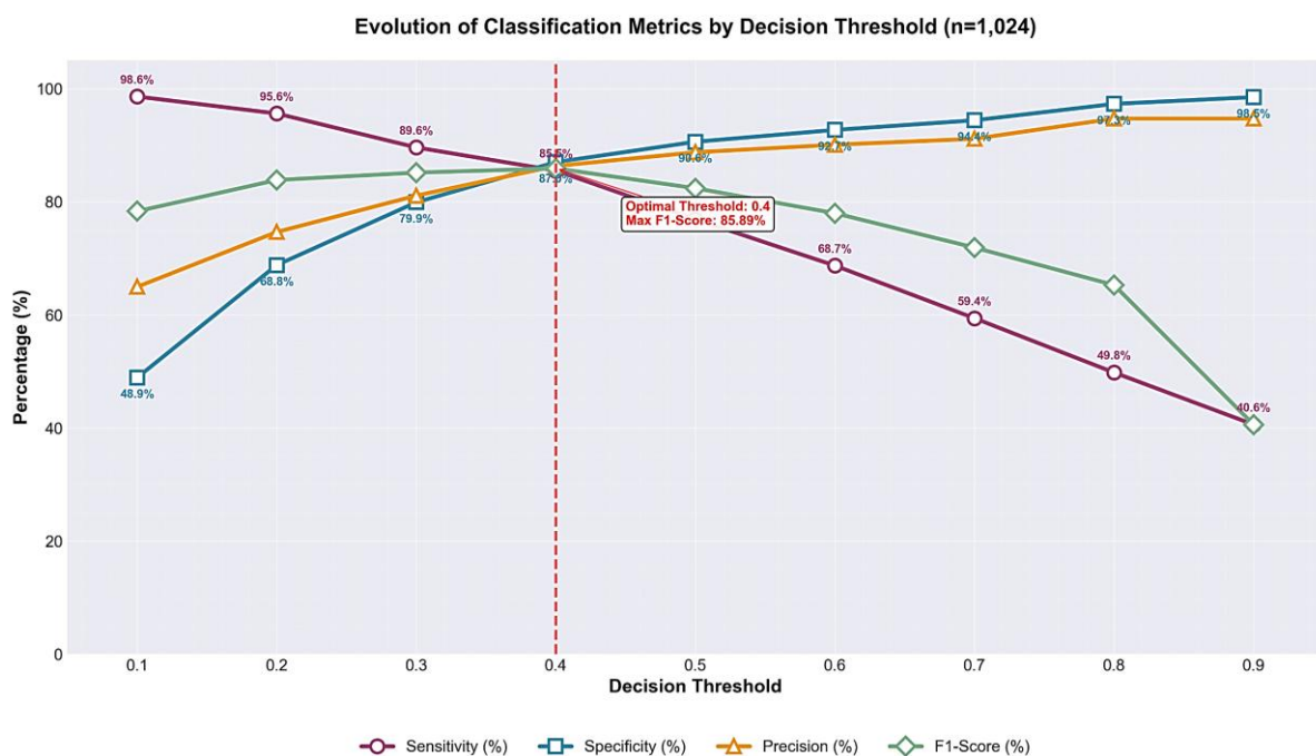
Figure 8. The evaluation matrices
