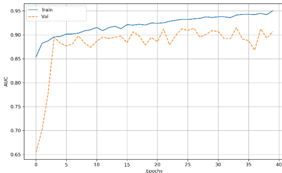
Figure 9. Comparison of learning curves (ablation)
