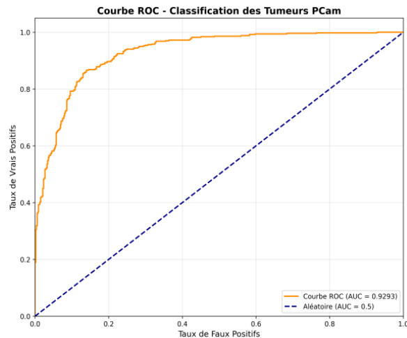
Figure 5. Roc curve
