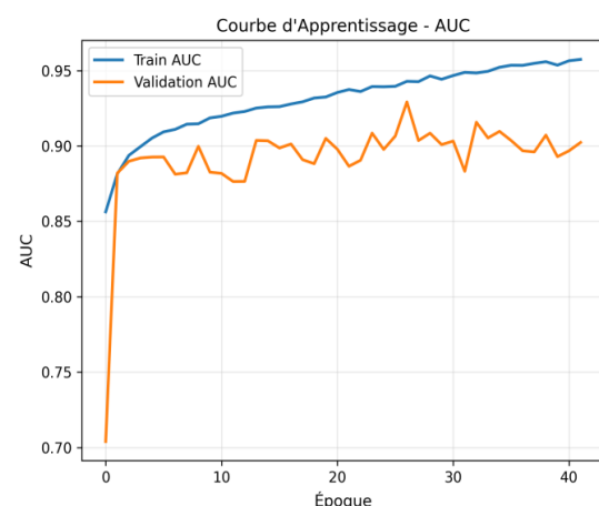
Figure 3. AUC learning curve
