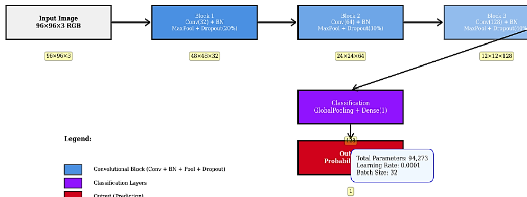
Figure 1. Simplified CNN architecture for breast tumor classification
