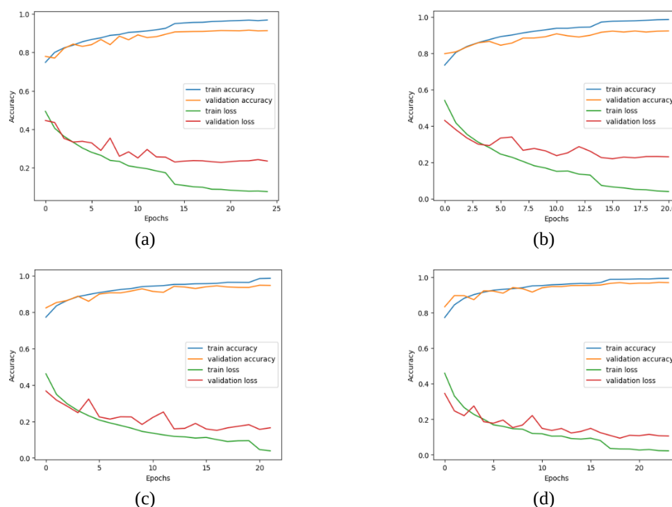
Figure 9. Training insights of (a) MobileNetV2, (b)Xception, (c) DenseNet169, and (d) ensemble model
