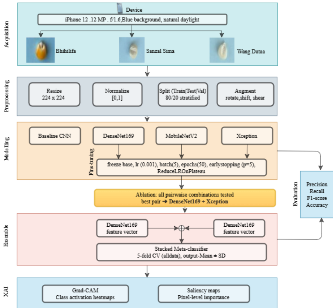
Figure 1. End-to-end pipeline for Ghanaian maize seed variety classification, from expert-verified RGB image acquisition through preprocessing, transfer learning, ensemble construction, five-fold cross-validation, and explainability analysis via Grad-CAM and saliency maps
