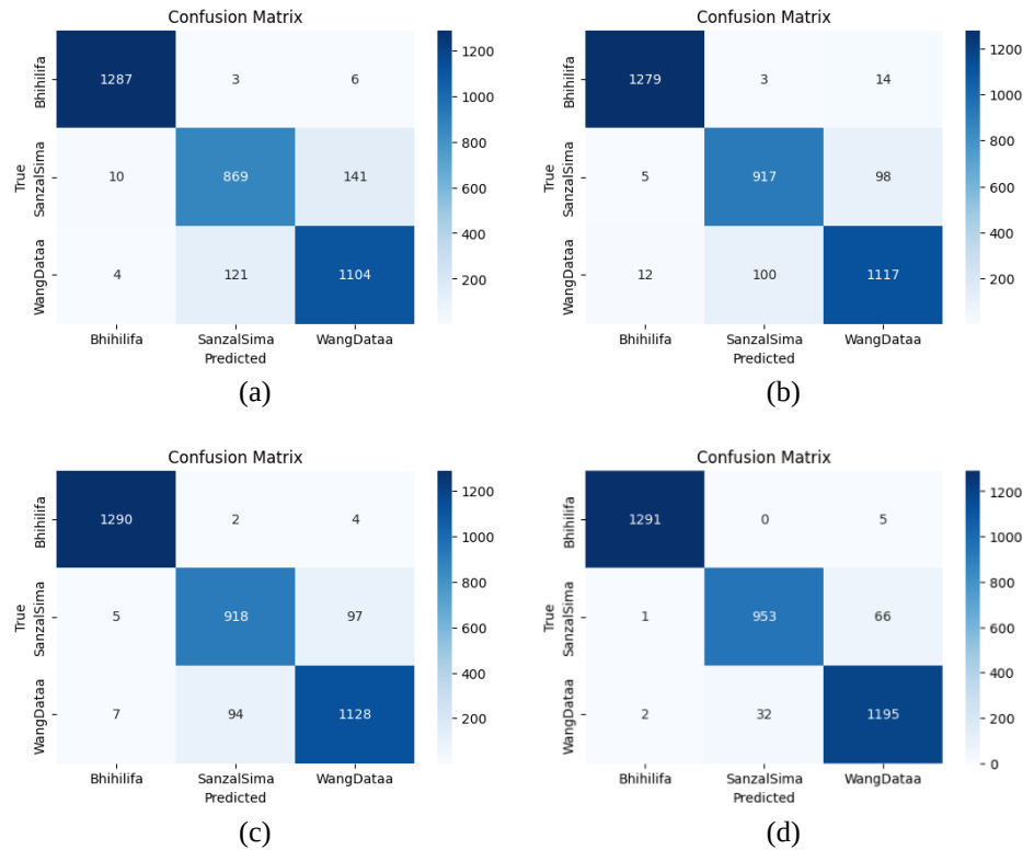
Figure 10. Confusion matrix of, (a) MobileNetV2, (b) Xception, (c) DenseNet169, and (d) ensemble model on test data
