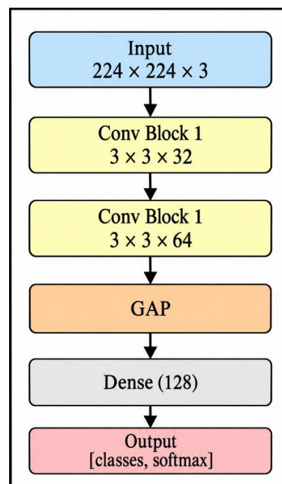
Figure 5. Baseline CNN architecture for Ghanaian maize seed variety classification
