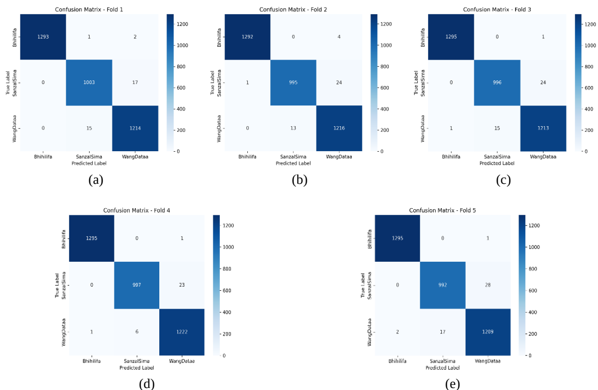
Figure 11. Confusion matrix of the ensemble model derived from 5-fold cross-validation (a) Fold 1, (b) Fold 2, (c) Fold 3, (d) Fold 4, and (e) Fold 5, illustrating consistent correct predictions across the three maize seed varieties (Bhihilifa, Sanzal Sima, and Wang Dataa)
