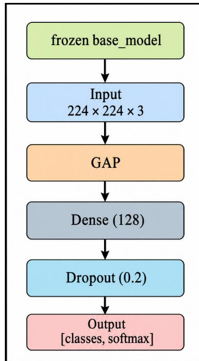
Figure 6. Fine-tuning pipeline for the pre-trained transfer learning architectures (DenseNet169, MobileNetV2, and Xception)
