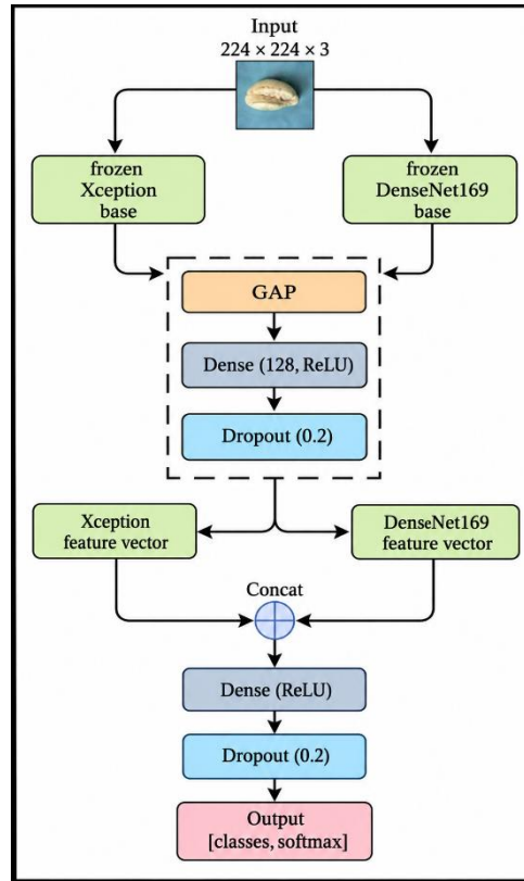
Figure 7. Proposed ensemble architecture combining DenseNet169 and Xception via feature concatenation and a stacked meta-classifier
