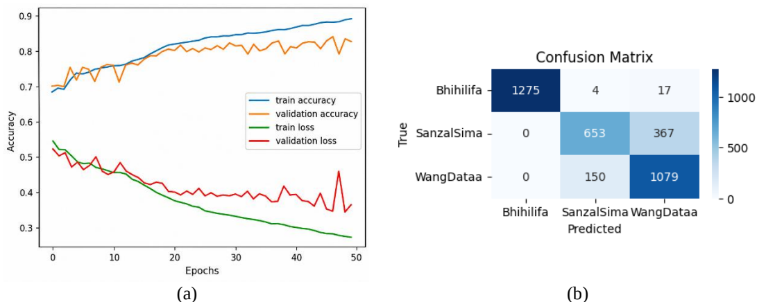
Figure 8. Baseline training curve (a) and confusion matrix and (b) on test set
